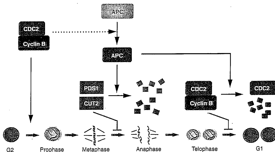
Fig. 3. Proteolysis at the metaphase-anaphase transition. A model is presented for how APC participates in the degradation of both mitotic cyclins and anaphase inhibitors. The model summarizes findings from various organisms. Although some substrates have been identified in only a single organism, the APC appears to have a universal role in mitotic proteolysis in eukaryotes. In this model, cyclin B accumulates during interphase to activate CDC2, producing an active mitotic CDK that triggers entry into prophase, resulting in the eventual formation of the mitotic spindle and metaphase plate. The mitotic CDK also leads to the activation of the APC by an undefined pathway. Once the APC is activated, it catalyzes the ubiquitination of several substrates, including the anaphase inhibitors PDS1 (budding yeast) and CUT2 (fission yeast). The APC also mediates proteolysis of cyclin B, which is universally required for exit from telophase.
