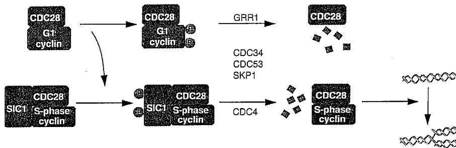
Fig. 2. A model for the regulated proteolysis of G1 cyclins and the CDK inhibitor SIC1 by the CDC34 pathway in budding yeast. G1 cyclins bind to CDC28 to produce an active G1 CDK complex. Phosphorylation of the G1 cyclin by CDC28 enables recognition of the G1 cyclin by components of the CDC34 pathway that ubiquitinate the protein and target it for degradation. The autocatalytic nature of the phosphorylation reaction makes G1 cyclins constitutively unstable. In contrast, the destruction of the CDK inhibitor SIC1 is cell-cycle dependent. SIC1 is stable during early G1 phase and prevents the precocious activation of S-phase CDKs. G1 CDKs assembled in late G1 phase phosphorylate SIC1, enabling its recognition and ubiquitination by components of the CDC34 pathway. The active S-phase CDK then initiates DNA replication by phosphorylating key substrates that remain to be identified. Whereas CDC34, CDC53, and SKP1 are required for degradation of both G1 cyclins and SIC1, GRR1 and CDC4 may be substrate-specific components of the destruction pathway (25).
