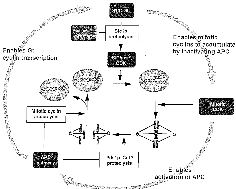
Fig. 4. How proteolysis drives the cell cycle. The model depicts a composite eukaryotic cell cycle and incorporates observations made in several different organisms. The chromosome cycle is depicted in the center of the figure, with interphase nuclei above and mitotic spindles below. The regulatory states of the cell cycle are interconnected by a series of dependencies. Each regulatory state has two functions: to trigger a chromosomal event such as replication, chromosome alignment, or segregation, and to enable the transition to a subsequent regulatory state (gray arrows). For example, G1 CDKs trigger DNA replication by activating S-phase CDKs through proteolysis and also enable mitotic cyclins to accumulate by inactivating the APC. Mitotic CDKs trigger chromosome condensation and spindle assembly, and also enable the activation of the APC. The active APC initiates anaphase by ubiquitinating anaphase inhibitors such as CUT2 and PDS1. The APC also catalyzes destruction of cyclin B, resulting in exit from mitosis, and enabling G1 cyclins to be resynthesized in the next cell cycle (116). The destruction of mitotic CDK activity is also required to allow formation of prereplication complexes (117), a prerequisite for DNA replication.
