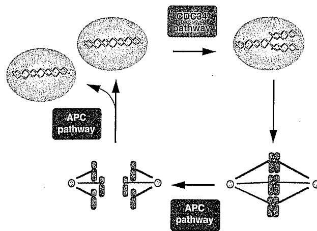
Fig. 1. Two distinct proteolytic pathways that participate in the regulation of the chromosome cycle. The nuclear cycle is depicted with a G1 phase nucleus in the upper left quadrant and an S phase nucleus on the right; mitotic spindles representing metaphase (right) and anaphase (left) are shown below. The CDC34 pathway promotes passage from G1 to S phase by degrading a CDK inhibitor. After chromosomes align at the metaphase plate, the APC pathway promotes the transition from metaphase to anaphase by degrading anaphase inhibitors, and subsequently promotes exit from mitosis by degrading mitotic cyclins.
